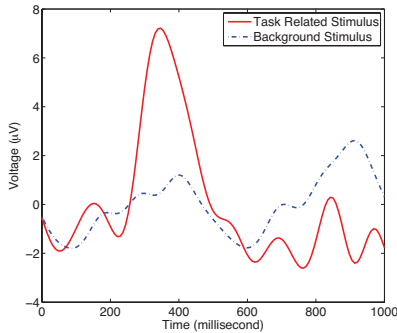
Figure 4: Multi-trial averaged bandpass filtered P300 signal from one electrode. The difference from the peak of the P300 signal to the background noise is about 6\mu V
