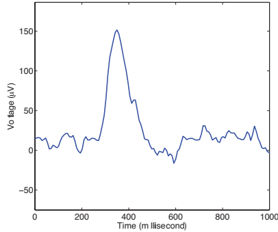
Figure 5: Unfiltered wink signal from one electrode. The difference from the peak of the wink signal to the background noise is about 140\mu V
