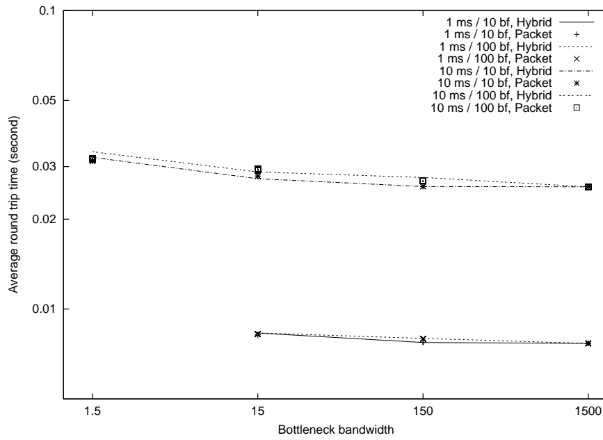
Figure 10: Latency Accuracy of Hybrid Model on Bottleneck Topology
