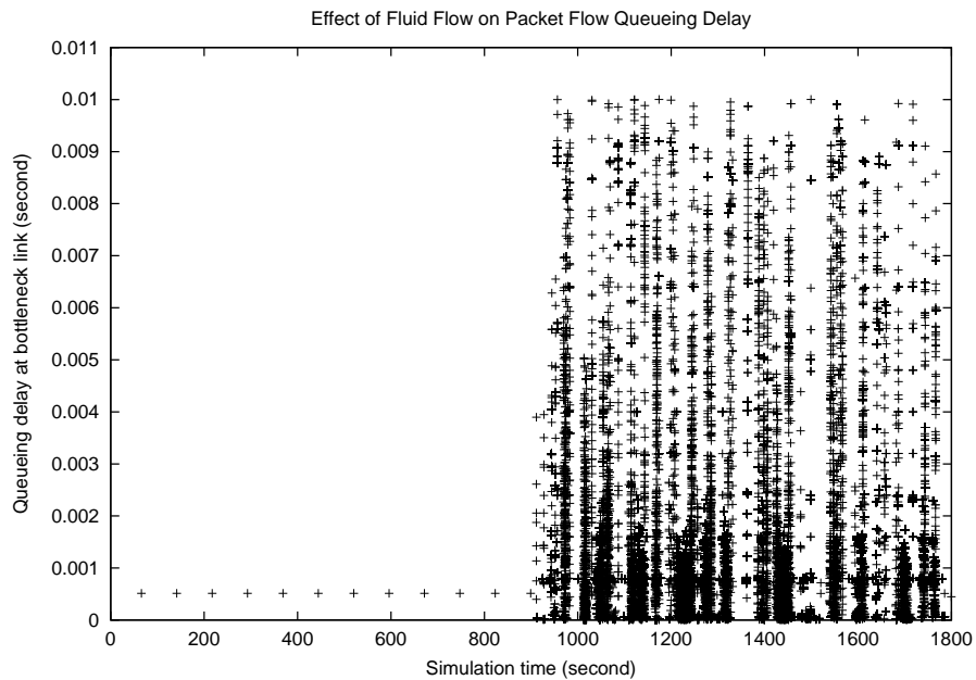
Figure 13: Interaction of Fluid and Packet Flows: Effects on Queuing Delay
