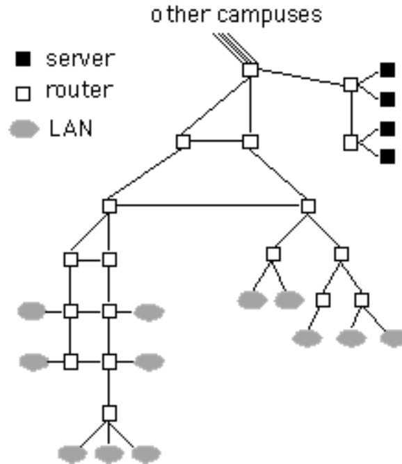
Figure 14: Topology of Campus
