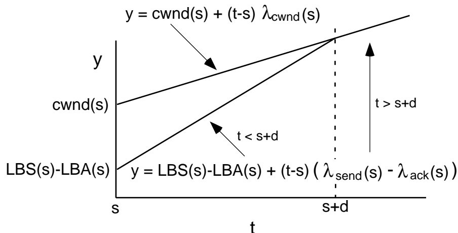
Figure 3: Point where LBS(t) - LBA(t) = cwnd(t) found by intersection of two linear functions
