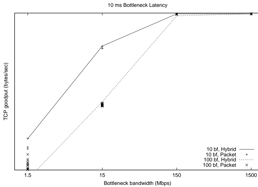
Figure 9: Loss and Goodput Accuracy of Hybrid Model on Bottleneck Topology, 10 ms Bottleneck Latency
