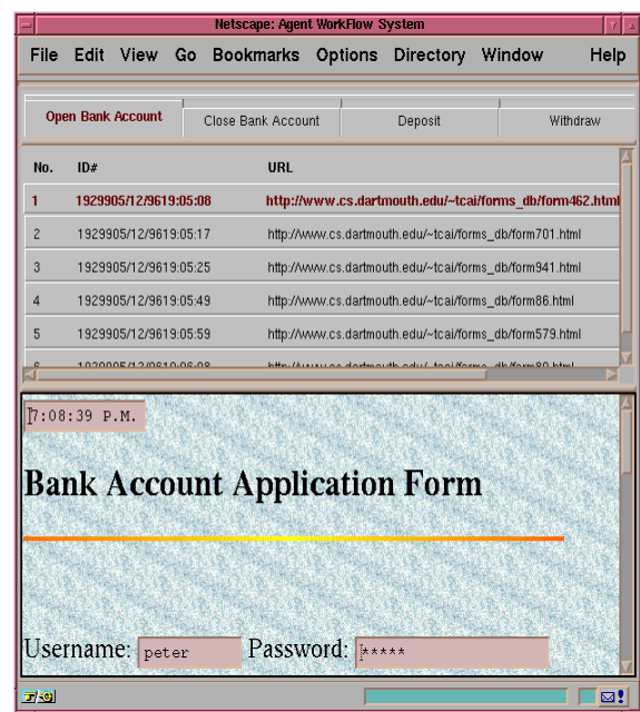
Figure 7 Worklist applet
