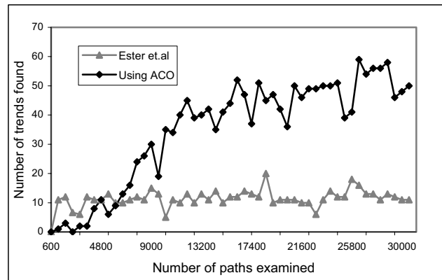
Figure 4: Comparison between the two algorithms
