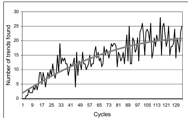
Figure 5: Improvement in Trend Discovery of Trend-Length=15
