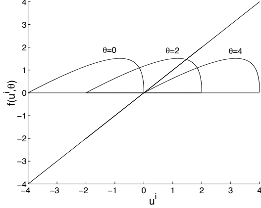
Figure 1. Behavior of \max(0, f_i(\theta - u_i^i)) for \alpha^i/\beta^i = 4
