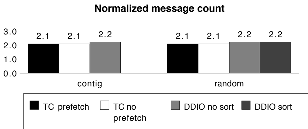
Figure 4: Normalized measures for experiments requesting an irregular subset of the file. Best execution time is computed from the peak disk bandwidth and the actual amount of data transferred. Best message count and message bytes are computed assuming that only the requested blocks will flow through the network.
