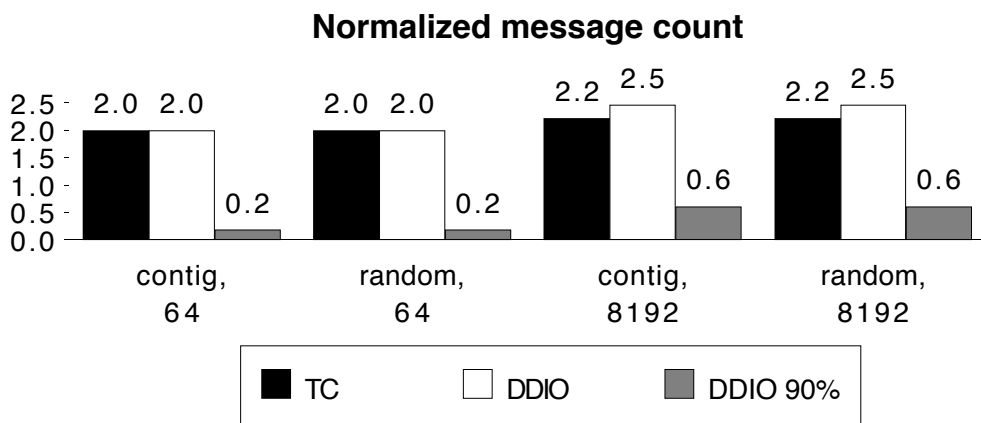
Figure 3: Results of data-dependent filtration experiments. Traditional caching is unchanged by filtering. We compare normal DDIO with a DDIO that filtered 90% of all records. The message metrics are normalized against the amount of traffic necessary with no filtration.
