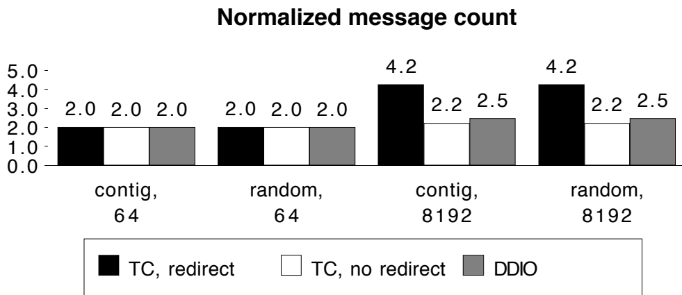
Figure 2: Results of data-dependent distribution experiments. Each graph is normalized against the “best” value for that measure. TC is traditional caching, and DDIO is disk-directed I/O. “contig” is a contiguous disk layout, and “random” is a random disk layout. Both 64- and 8192-byte records were used.
