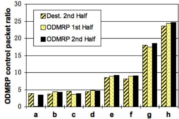
Fig. 6. ODMRP Control Packet Ratio
