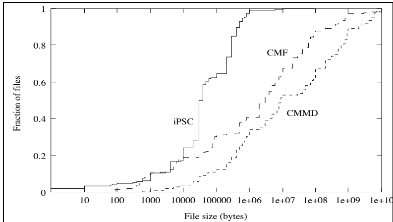
Figure 3: Cumulative distribution function (CDF) of the number of files of each size at close. For a file size x , CDF(x) represents the fraction of all files that had x or fewer bytes.
