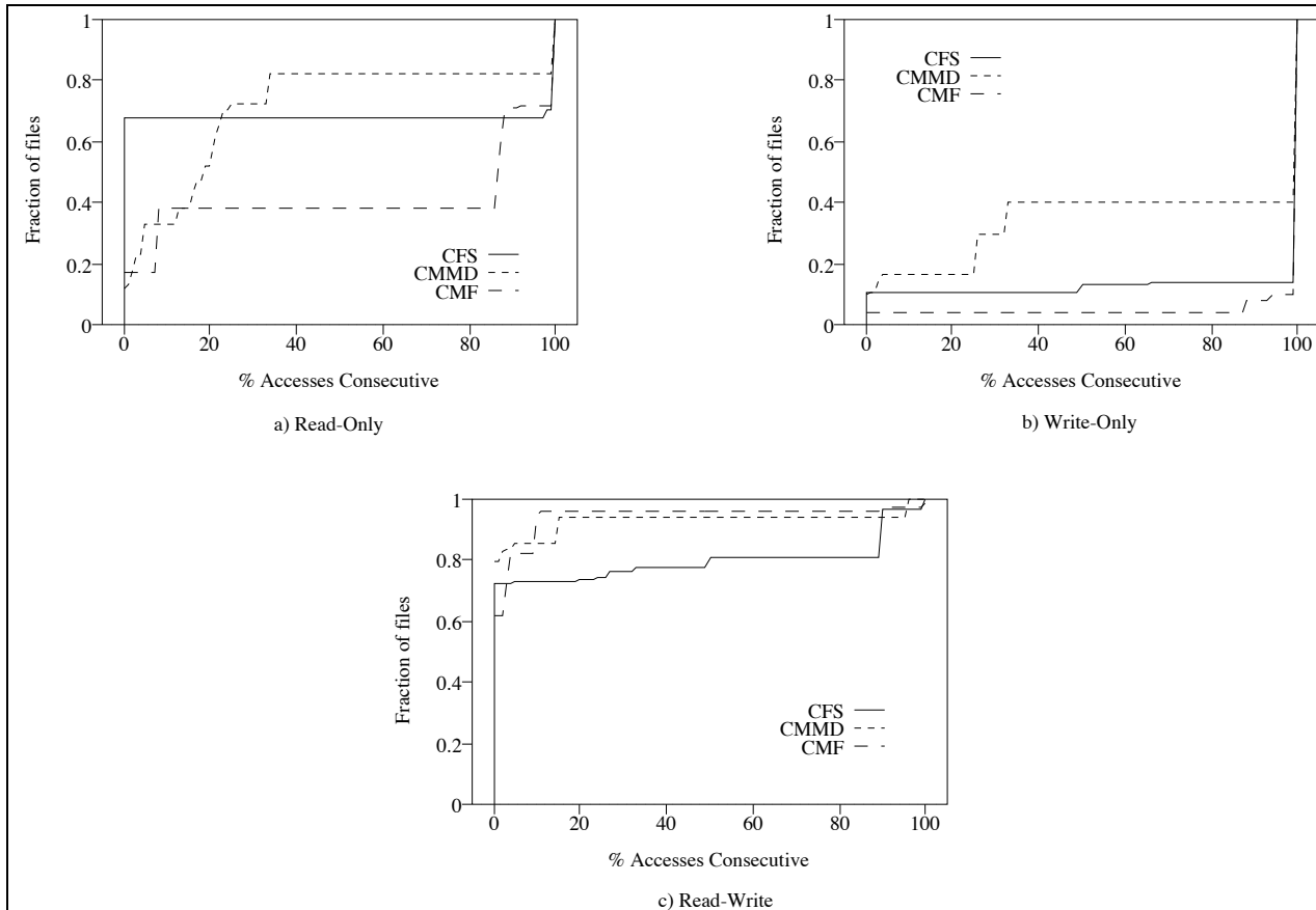
Figure 7: CDF of consecutive access to files. Each point on a line indicates the fraction of files in the workload that contain no more than the indicated percentage of consecutive accesses.
