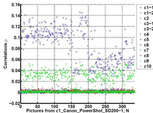
Figure 16. Identification of low resolution ( 1024 \times 768 ) c1 Canon SD200-1 images.
