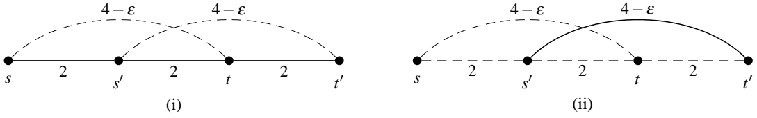
Figure 4: Instance used in the lower bound argument.
