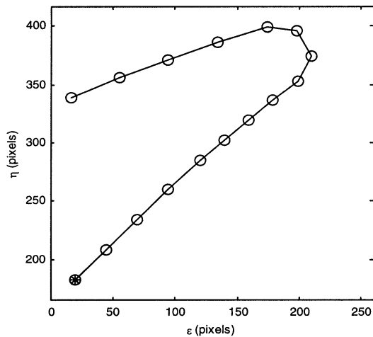
Fig. 8. Simulated fish track 1 of a fish performing a sharp U-turn. The graph axes are camera pixel coordinates. ○ represents a measurement, and * represents the start of the track.
