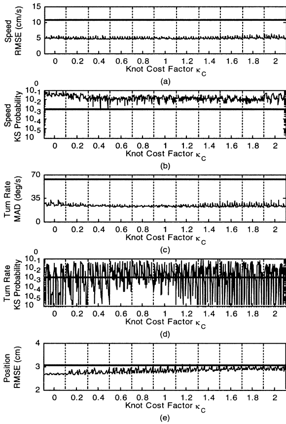
Fig. 4. STI performance and tuning sensitivity plot. The five plots show the STI's performance and sensitivity to five performance metrics. (a) Speed RMSE. (b) Speed KS probability. (c) Turn rate MAD. (d) Turn rate KS probability. (e) Position RMSE. The horizontal bars represent the baseline performance: values obtained without filtering for (a), (c), and (e), and the desired 0.01 probability level for (b) and (d). Lower values are better for (a), (c), and (e), while higher values are better for (b) and (d). Tuning parameters were iteratively varied using nested for-loops, first \kappa_C , then \tau , \kappa_\psi , and finally \kappa_\sigma .
