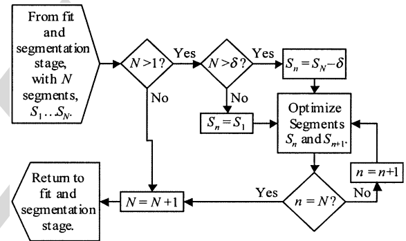
Fig. 2. STI recursive optimization stage flowchart.
