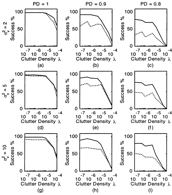
Fig. 10. Percentage of 100 Monte Carlo simulations of track 1 (Fig. 8) where the target was successfully tracked from start to finish for various levels of Poisson clutter density parameter \lambda , probability of detection (PD), and measurement noise variance \sigma_v^2 (in pixels 2 ). Solid line is the STIJPDAF; dashed line is the EKFPDAF. (a) PD = 1, \sigma_v^2 = 2 . (b) PD = 0.9, \sigma_v^2 = 2 . (c) PD = 0.8, \sigma_v^2 = 2 . (d) PD = 1, \sigma_v^2 = 5 . (e) PD = 0.9, \sigma_v^2 = 5 . (f) PD = 0.8, \sigma_v^2 = 5 . (g) PD = 1, \sigma_v^2 = 10 . (h) PD = 0.9, \sigma_v^2 = 10 . (i) PD = 0.8, \sigma_v^2 = 10 .
