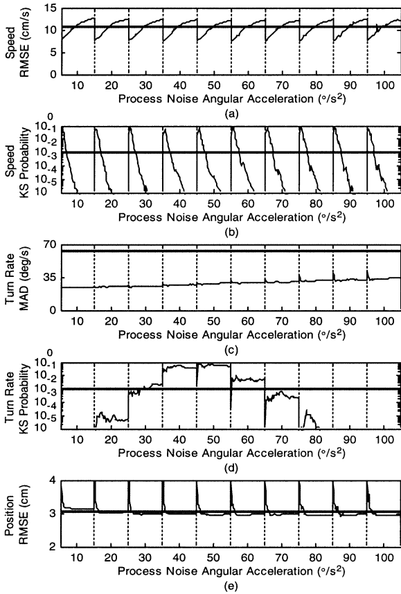
Fig. 6. EKF performance and sensitivity tuning sensitivity plot. Format is the same as Fig. 4. Tuning parameters were iteratively varied using nested for-loops, first process noise angular acceleration, and then process noise tangential acceleration.
