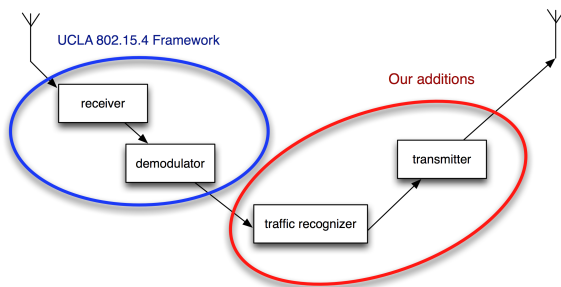
Figure 7. Selective Jamming Architecture on USRP2
