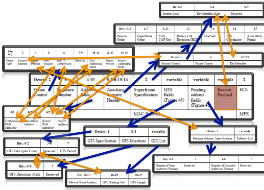
Figure 3. Relationships and dependencies between fields in 802.15.4 Beacon Frames
