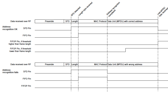
Figure 5. Chipcon 2420 Receive Operation Pin Values [32, 34]
