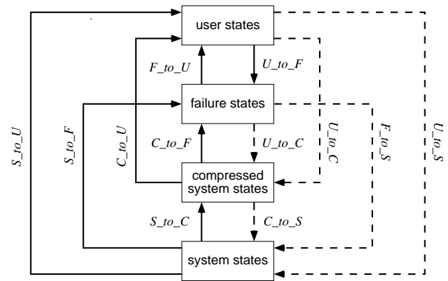
Figure 3. Maps take states across levels; dashed lines indicate one-to-many maps.
