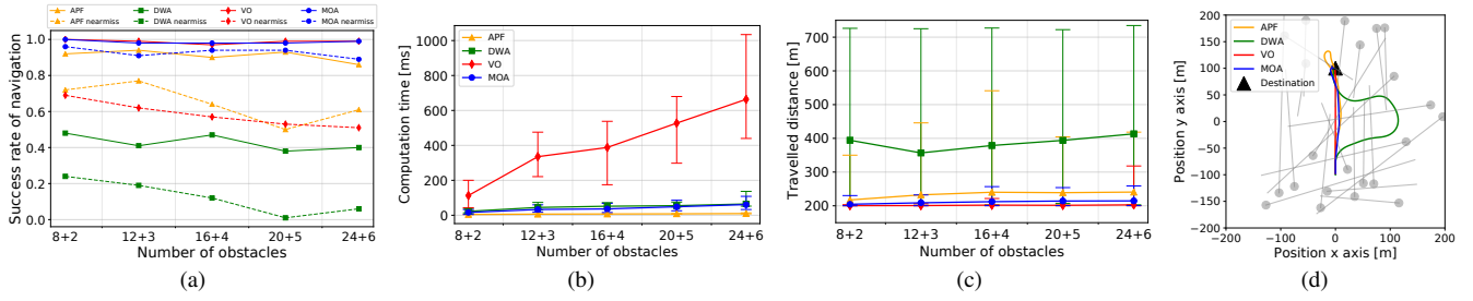
Fig. 5. Comparison of each method for collision avoidance of multiple obstacles under congested traffic. (a) Success rate of navigation. Solid : success rate without consideration of near miss area entrance, Dotted : success rate with near miss area entrance regarded as collision ; (b) Computational time; (c) Travelled distance of ASV when the navigation task was successful; and (d) Trajectories in an example scenario with 30 obstacles (gray).
