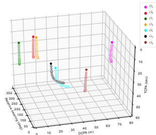
Fig. 3. Motion attributes – TCPA, DCPA, relative bearing – by multiple obstacles under congested traffic in Fig. 1 scenario. The three attributes are monitored with respect to the controlled ASV ( R ) while it is assumed that obstacles do not take an evasive action.
