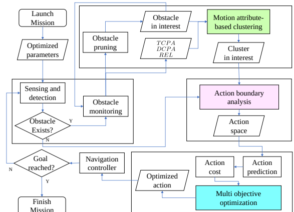
Fig. 2. Obstacle avoidance pipeline overview.
