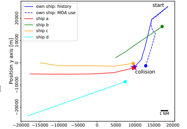
Fig. 7. Trajectories of ships during 1.5 hours prior to a collision off coast Japan. Southwest-bound ship ( solid blue ) collided with East-bound ship a while the proposed method successfully avoided all the ships ( dotted blue ) in the same scenario. Note that the involved vehicles were made anonymous.
