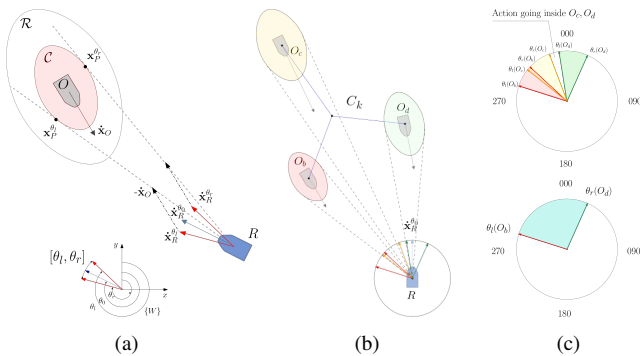
Fig. 4. Geometric representation of action boundary for obstacle(s) and cluster. (a) conceptual diagram of an action boundary in a single obstacle. (b) boundary analysis for multiple obstacles with varying ship domain sizes in the cluster C_k in Fig. 1 example. (c) top: boundary analysis result for each cluster; bottom: holistic analysis proposed by this study identifies determinant obstacles as O_b, O_d such that [\theta_l(O_b), \theta_r(O_d)] encompasses the action boundaries of the obstacles in the cluster.
