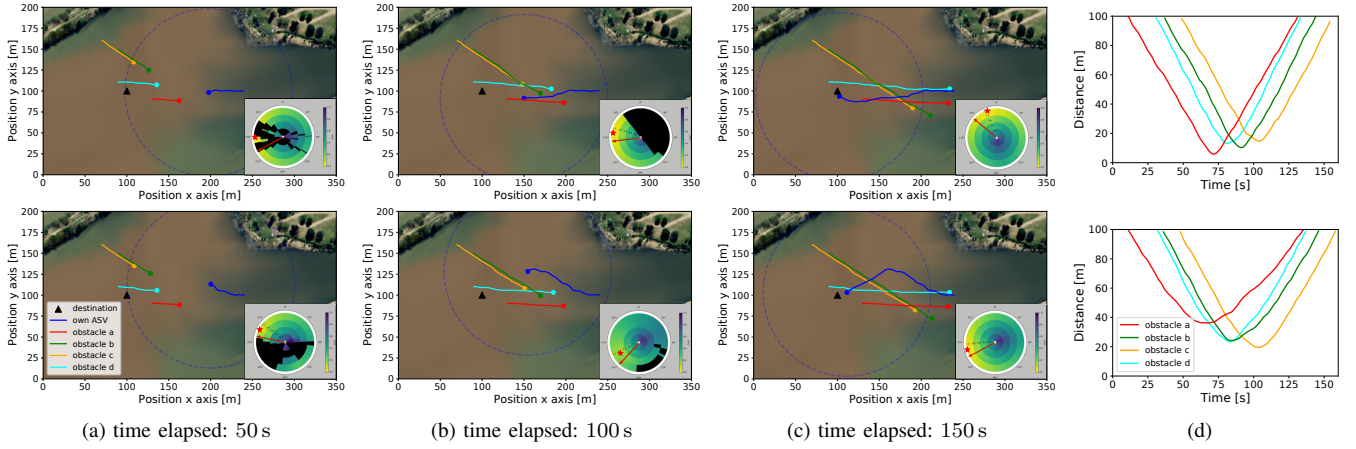
Fig. 6. Comparison of trajectories and action spaces by the-state-of-the-art VO ( top ) vs the proposed MOA ( bottom ) method for collision avoidance of multiple obstacles in Porto Alegre, Brazil with locally varying water/wind currents. The controlled ASV ( Blue ) with length 4 m, max speed 1 m/s departed from the river mouth (250, 100) to the open waters (100, 100), while the obstacles merged with arrival traffic. In the action space, red star and red line represents the best action and current action, respectively. (a) VO attempted to go between obstacle a , d . MOA proactively took a right-side action while obstacle a , b , d were clustered. Note that obstacle d was under tracking process as it just entered the sensible range 100 m; (b) VO passed the obstacles, particularly in very close proximity to obstacle a , b . MOA safely passed obstacles. Note that clusters were adaptively identified, e.g., obstacle ( a , b , d ) to obstacle ( a , d ) and ( b , c ) based on changes of motion attributes; (c) VO arrived at the destination. MOA cleared obstacles while still proceeding to the destination; and (d) Distance comparison shows MOA avoid obstacles under congested traffic in a safer manner.
