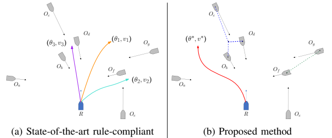
Fig. 1. Collision avoidance behavior for controlled ASV, R , using state-of-the-art vs. proposed method under congested traffic with multiple obstacles O : (a) a desired action (\theta_1, v_1) complies with a left-to-left maneuver for the head-on O_b, O_c, O_d , while the bow-crossing maneuver conflicts with the crossing O_f, O_g ; (\theta_2, v_2) complies with a stern-crossing maneuver for the crossing O_f, O_g , while the change of action conflicts with stand-on status for overtaking O_e ; (\theta_3, v_3) partially complies with a left-to-left maneuver for the head-on O_b, O_c except O_d , while it leads to entering between the obstacles. (b) (\theta^*, v^*) achieves a safe and adaptive maneuver with only one bow-crossing for O_a , while clusters (O_b, O_c, O_d) and (O_f, O_g) are identified based on similar motion attributes with respect to R such that R will not pass areas (dotted lines) between obstacles in a cluster.
