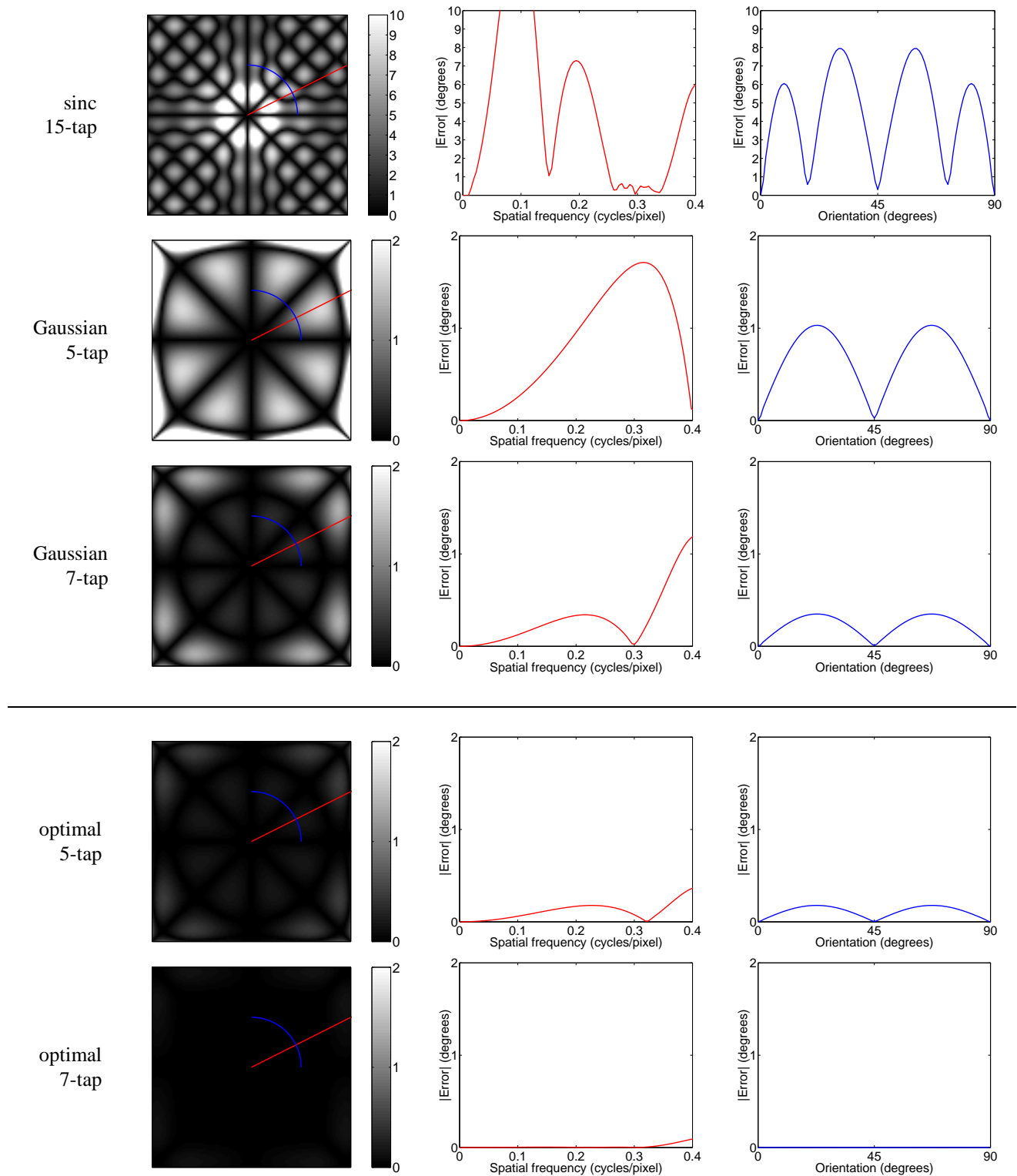
Fig. 6: First-order derivatives: errors in estimating the orientation of a sinusoidal grating of varying spatial frequencies and orientations (see caption of Fig. 5). Note that the scaling of the truncated sinc filter errors is different than the others.
