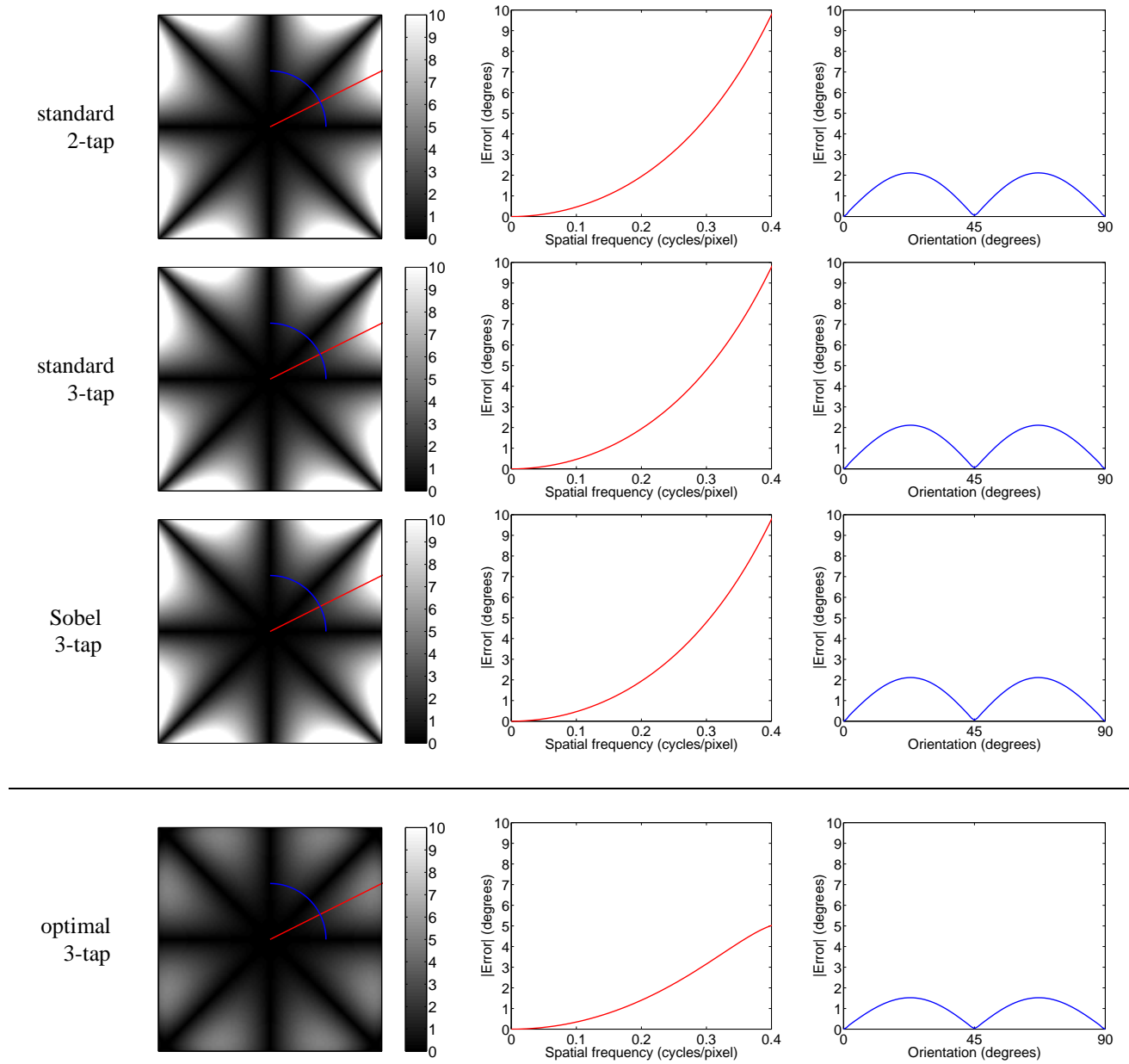
Fig. 5: First-order derivatives: errors in estimating the orientation of a sinusoidal grating of varying spatial frequencies and orientations. The intensity image in the left column shows the orientation error (brighter pixels correspond to larger errors) across all spatial frequencies - the axes span the range [-\pi, \pi] . The plots in the second and third columns correspond to the indicated radial and angular slices through this two-dimensional frequency space.
