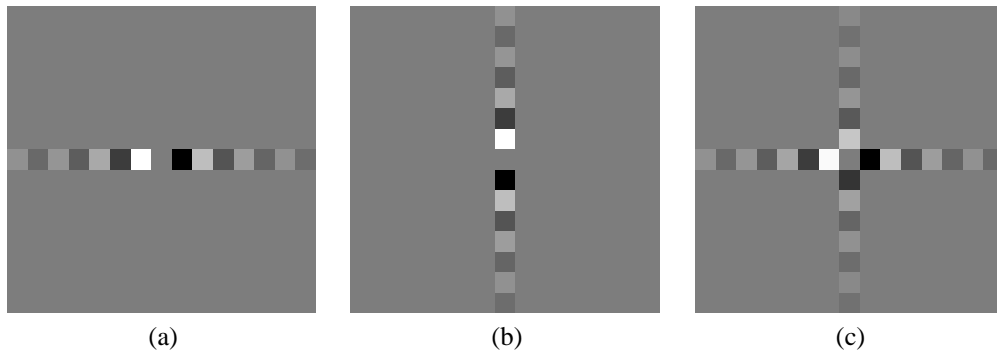
Fig. 2: Illustration of sinc-based two-dimensional differentiators. Shown are (a) horizontal; (b) vertical; and (c) oblique (30 degrees) differentiation filters. The last of these is constructed from a linear combination of the on-axis filters, as specified by Eq. (9).
