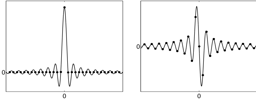
Fig. 1: The ideal interpolator (sinc) function (left) and its derivative (right). Dots indicate sample locations.
