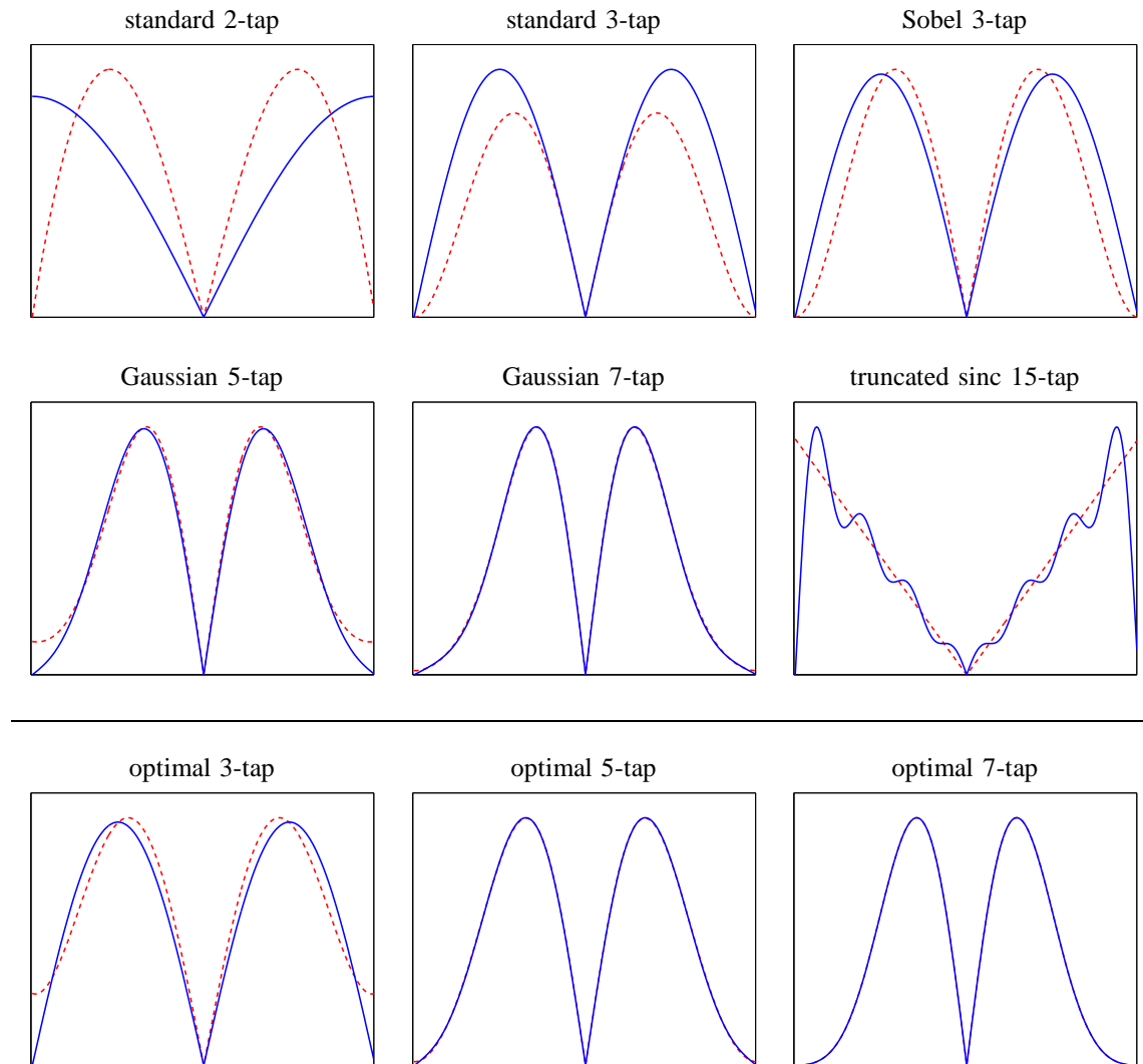
Fig. 4: First order derivatives: Fourier magnitude, plotted from -\pi to \pi . The dashed red line corresponds to the product of a ramp and prefilter, and solid blue line corresponds to the derivative filter.
