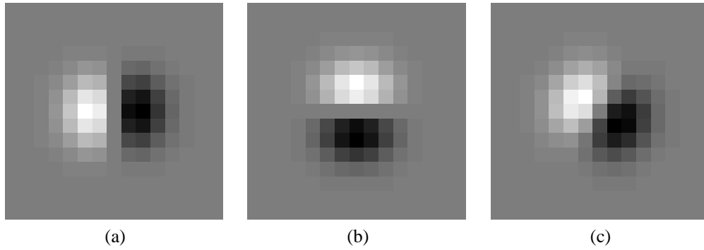
Fig. 3: Shown are (a) horizontal; (b) vertical; and (c) oblique (30 degrees) differentiation filters. The last of these is constructed from a linear combination of the on-axis filters, as specified by Eq. (9). These filters should be compared with those of Fig. (2).
