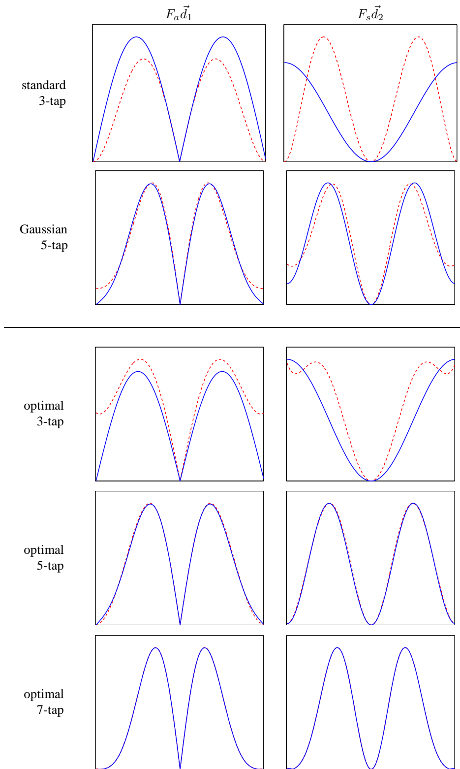
Fig. 7: Second-order derivatives: Fourier magnitudes, plotted from -\pi to \pi . Left side shows first-order filter (solid blue), compared with product of a ramp and the prefilter (dashed red). Right side shows second-order filter compared with product of squared ramp and prefilter.
