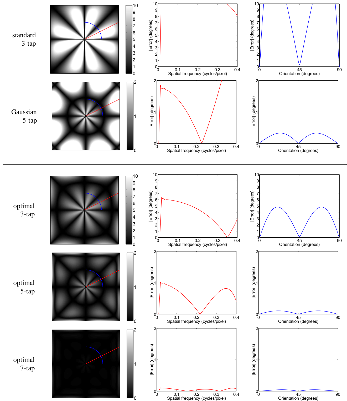
Fig. 8: Second-order derivatives: errors in estimating the orientation of a sinusoidal grating of varying spatial frequencies and orientations. Note that the scaling of the 3-tap filter's errors are different than the others.
