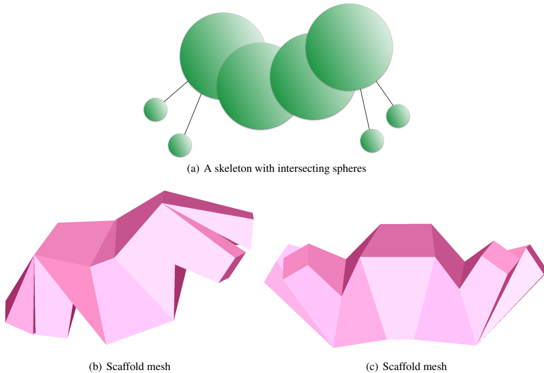
Fig. 8 The simple skeleton of Figure 7 with varying radii. The large radii lead to intersecting spheres at the interior vertices, but the faces remain quads.
