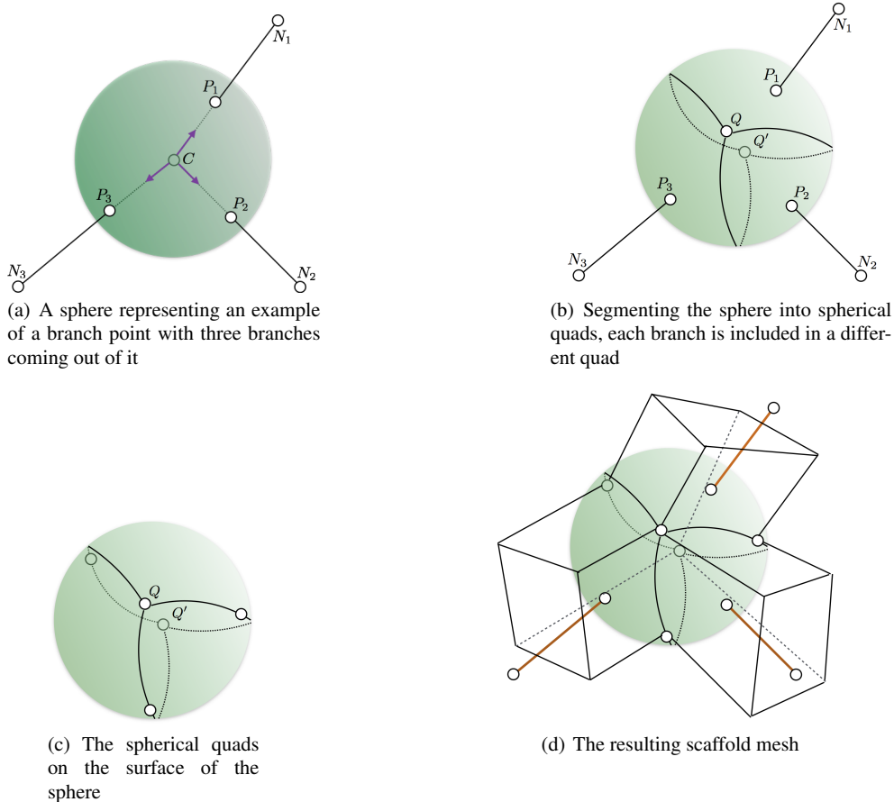
Fig. 3 A sphere with centre C , neighbors \{N_1, N_2, N_3\} and resulting points of intersection on the sphere \{P_1, P_2, P_3\} (a). The segmentation of the sphere into sections (b). The addition of points along the geodesics to create the quadrilaterals (c). The scaffold mesh (d).
