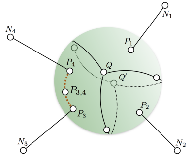
(a) The sphere of Fig. 3(c) with an added branch.
