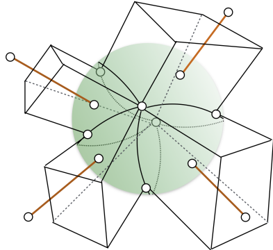
(b) The resulting scaffold mesh of Fig. 4(a)
