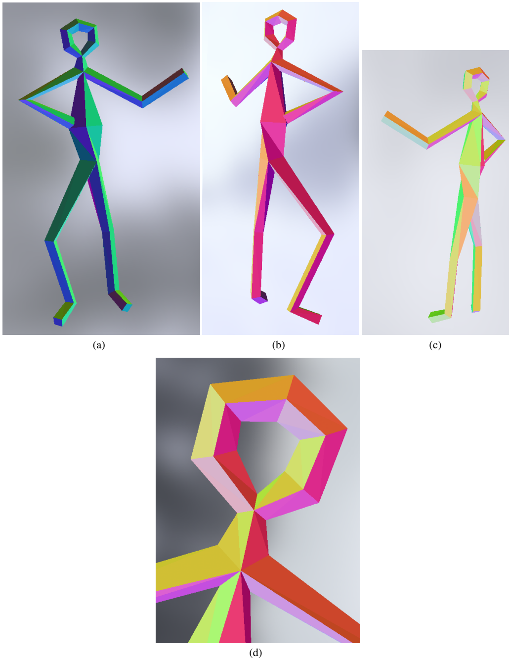
Fig. 9 The scaffold mesh created from the skeleton in Figure 1; all faces of the mesh are quads, as well as the section of any sleeve.
