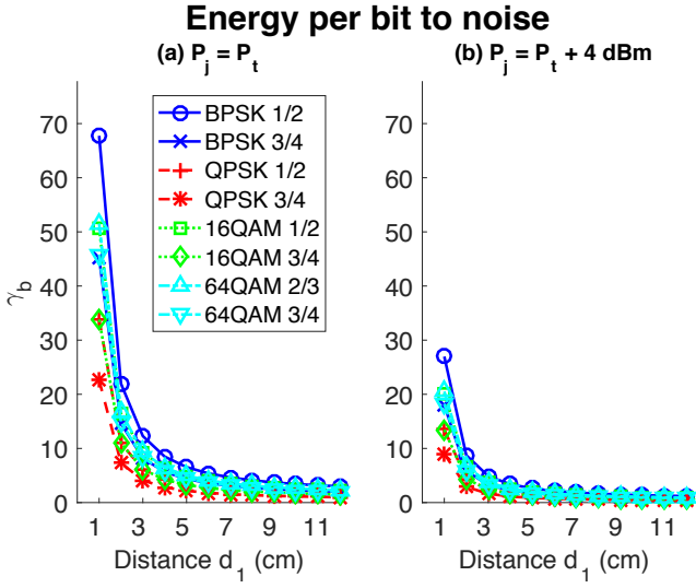
Figure 4: Energy per bit vs. noise at close range.
