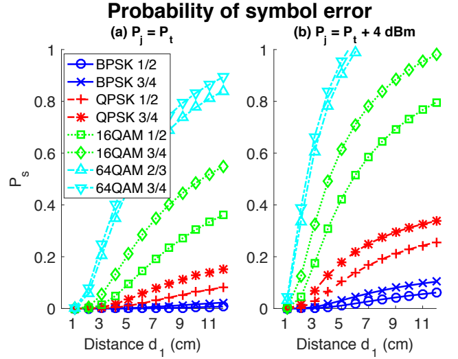
Figure 5: Probability of symbol error by MCS for devices in close proximity.
