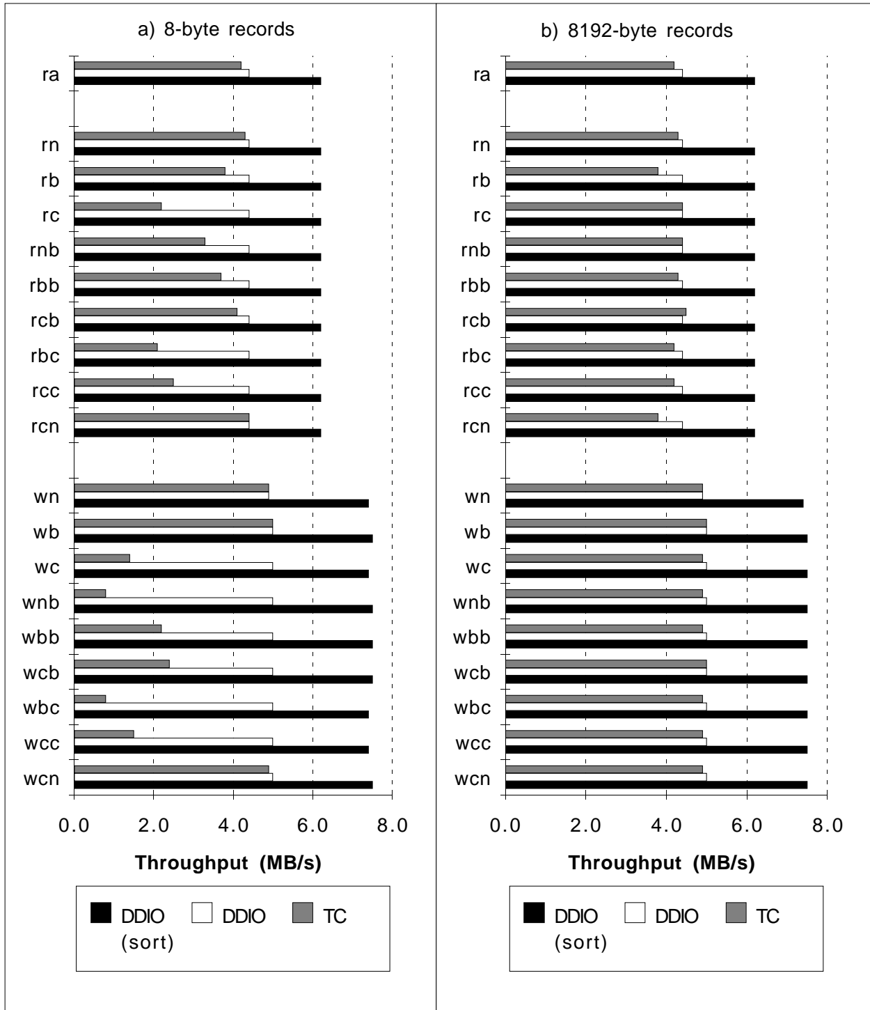
Figure 3: Two graphs comparing the throughput of disk-directed I/O (DDIO) to that of traditional caching (TC), on a random-blocks disk layout. r_a throughput has been normalized by the number of CPs. Each point represents the average of five trials of an access pattern on both methods (maximum coefficient of variation ( cv ) is 0.14).
