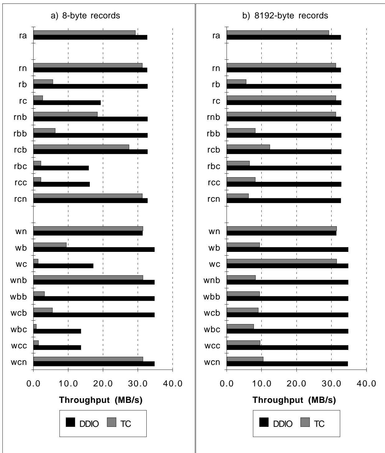
Figure 4: Two graphs comparing the throughput of disk-directed I/O (DDIO) and traditional caching (TC), on a contiguous disk layout. r_a throughput has been normalized by the number of CPUs. Each point represents the average of five trials of an access pattern on both methods (maximum cv is 0.13). Note that the peak disk throughput was 37.5 Mbytes/s.
