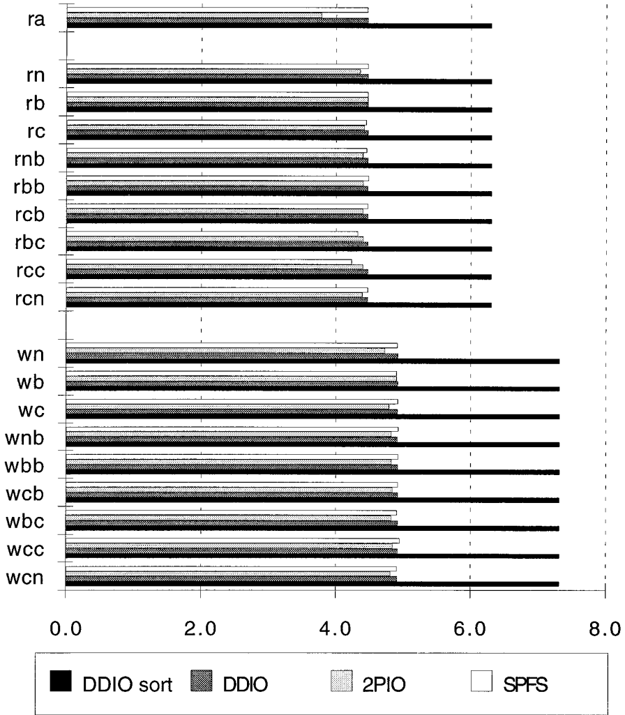
Fig. 5. Comparing the throughput of disk-directed I/O (DDIO) to that of two-phase I/O (2PIO) and the simple parallel file system (SPFS), on a random-blocks disk layout using patterns with an 8192-byte record size. ra throughput has been normalized by the number of CPs. Each point represents the average of five trials of an access pattern (the maximum cv is 0.031).
