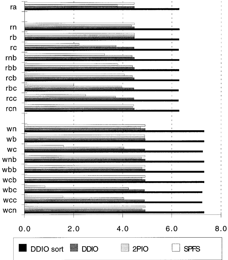
Fig. 4. Comparing the throughput of disk-directed I/O (DDIO) to that of two-phase I/O (2PIO) and the simple parallel file system (SPFS), on a random-blocks disk layout using patterns with an 8-byte record size. ra throughput has been normalized by the number of CPs. Each point represents the average of five trials of an access pattern (the maximum coefficient of variation ( cv ) is 0.042, except for 0.32 on wc on SPFS).
