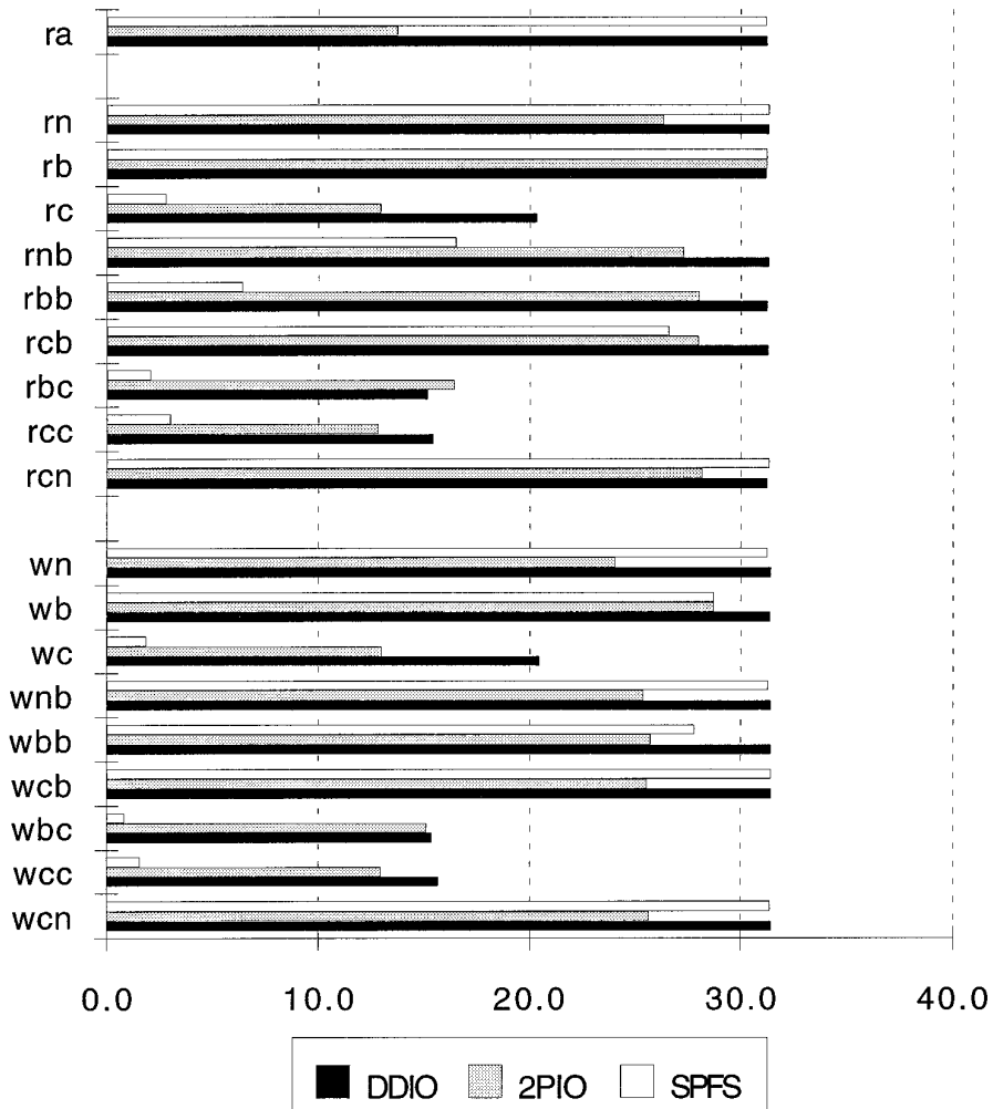
Fig. 6. Comparing the throughput of disk-directed I/O (DDIO), two-phase I/O (2PIO), and the simple parallel file system (SPFS), on a contiguous disk layout, using access patterns with 8-byte records. Note that “DDIO” and “DDIO sort” are identical here, because the logical block numbers are identical to the physical block numbers, so the sort is a no-op. ra throughput has been normalized by the number of CPUs. Each point represents the average of five trials of an access pattern (the maximum cv is 0.052, except for 0.25 on 8-byte wc on SPFS). Note that the peak disk throughput was 33.8MB/s.
