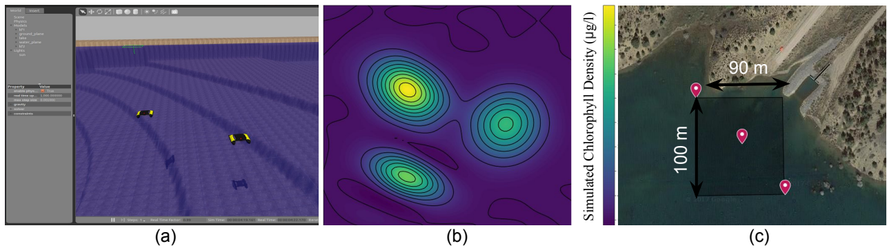
Fig. 5. (a) Gazebo simulation for the ASV [23] used in our experiments. (b) Simulated chlorophyll density map overlaid on top of the water surface. The colorbar shows the simulated chlorophyll density. (c) Part of the Lake Nighthorse, Durango used for running simulation experiments.
