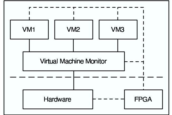
Figure 3: A Block Diagram of the proposed architecture. The bold lines indicate traditional VM interactions and the dotted lines indicate interactions with the FPGA.
