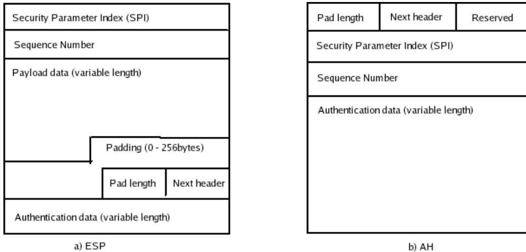
Figure 2.1.2-1: IPsec information part of IP packet
