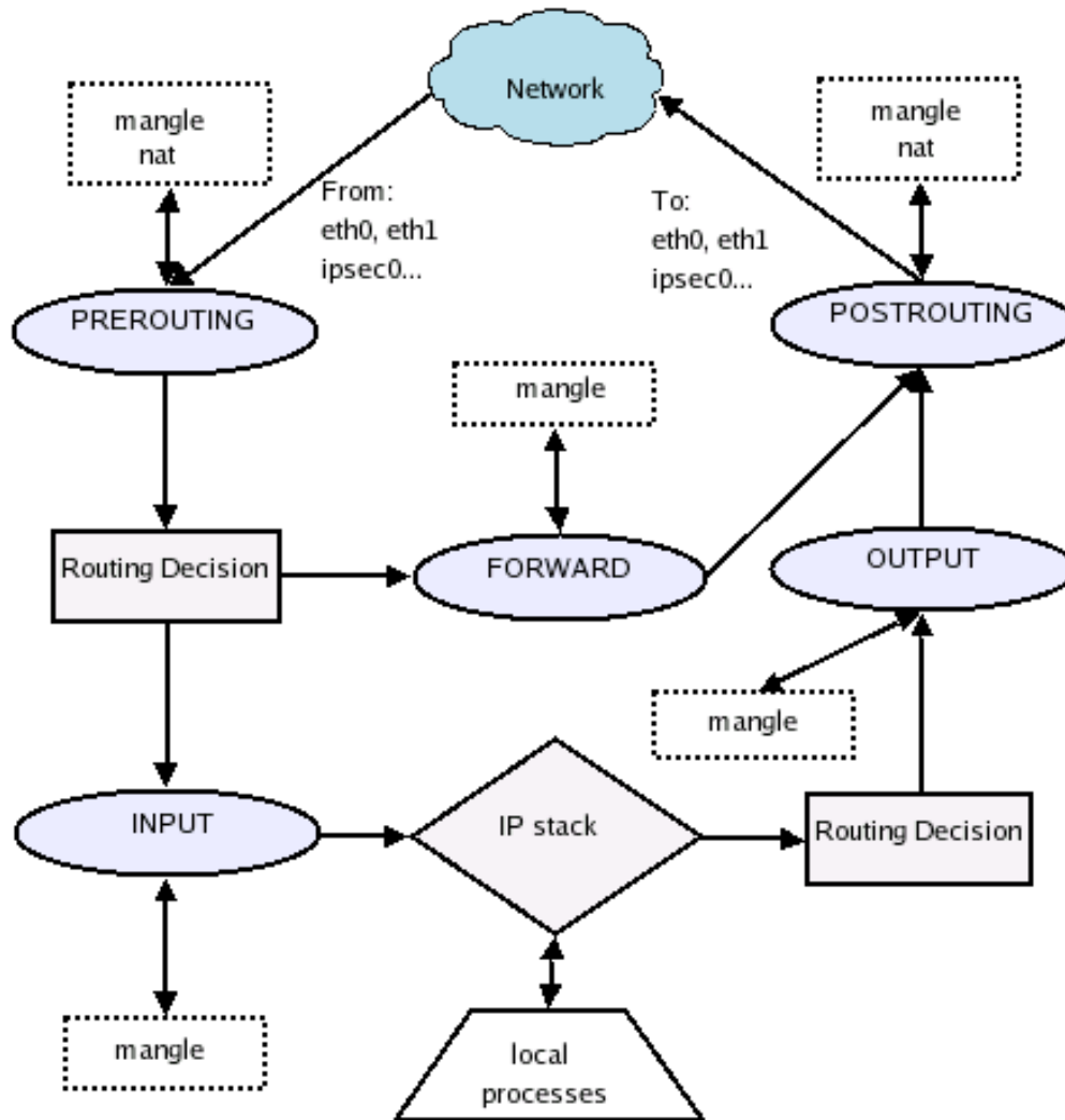
Figure 2.3.1-1: Iptables chains and tables
