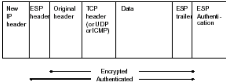
Figure 2.1.2-2: IPsec using ESP in Tunnel Mode
