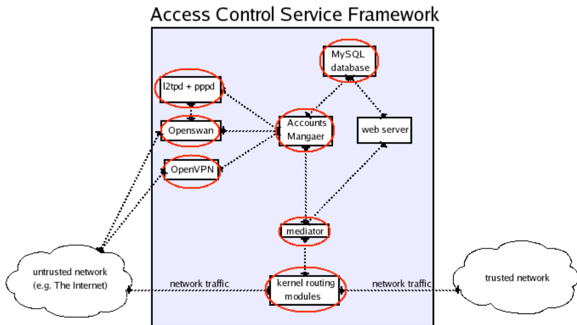
Figure 3.3-1: Design for ACS prototype. The circled components are those installed or programmed in my implementation. The dotted lines between components represent communication, usually by passing messages.
