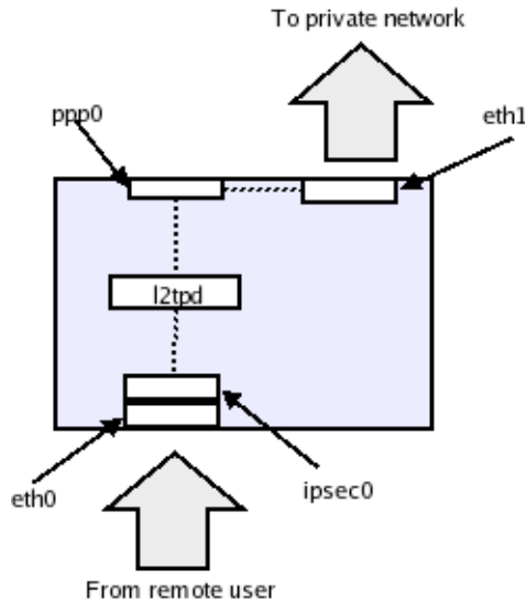
Figure 3.3.1-1: Linux VPN Server setup using pppd, user-land l2tp daemon and Openswan IPsec tool.
