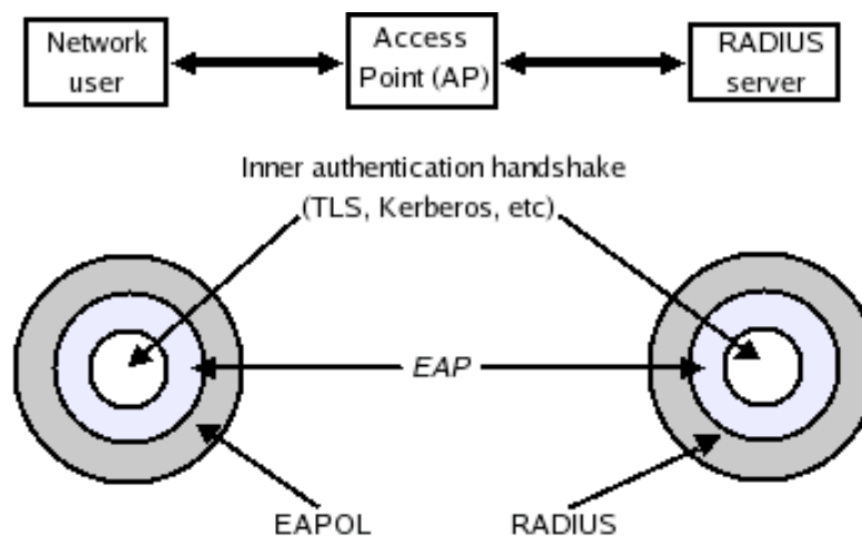
Figure 2.4-1: A network user requests permission to join the network. In 802.1x terminology the network user is a supplicant , the AP is an authenticator , and the RADIUS server as an authentication server . The user and AP communicate by EAPOL while the AP and RADIUS use the RADIUS protocol. Both protocols encapsulate EAP messages that, in turn, encapsulate some other authentication protocol such as TLS. This figure is a re-creation of a diagram from Goffee’s thesis on the same subject [Goff04]. Kwang-Hyun Baek put forward the concept for the diagram.
